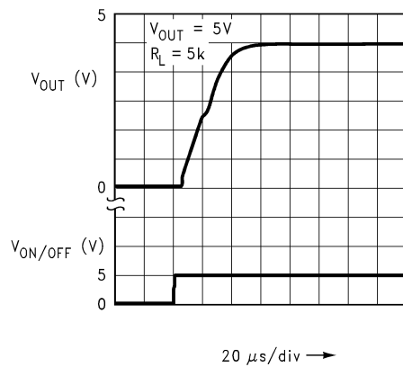
Turn-On Waveform
