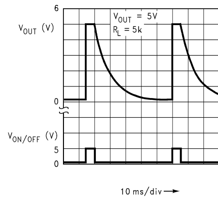
Turn-Off Waveform
