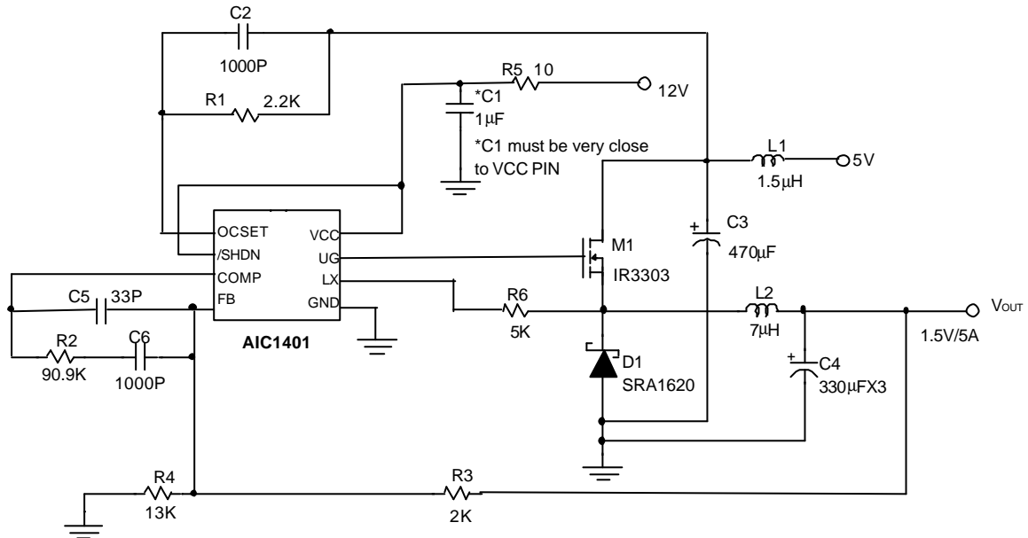
DC/DC Converter
