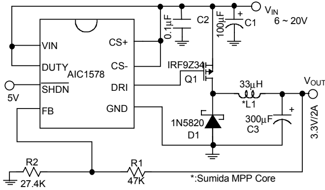
Fig. 2 3.3V Step-Down Converter
