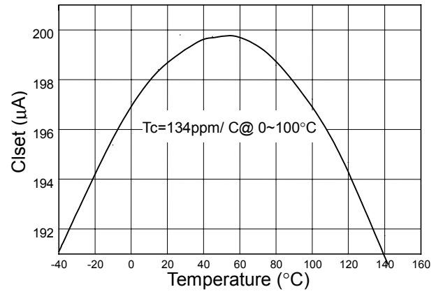
OCSET Current vs. Temperature
