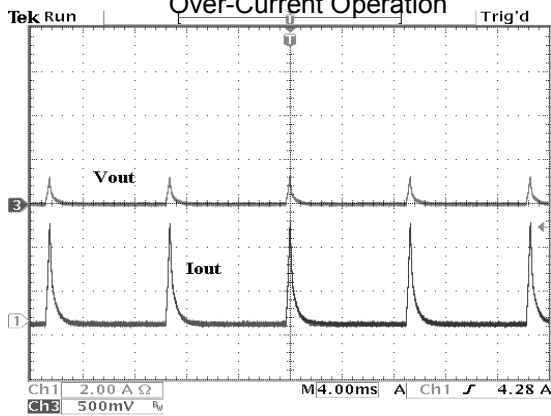
Over-Current Operation
