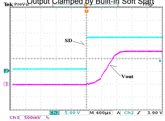
Output Clamped by Built-In Soft Start
