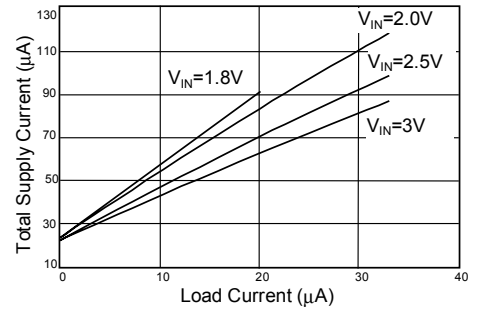
Fig. 6 Low Supply Current Burst Mode Step-Up Converter
