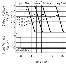
Input Overdrive Referenced to V_{OS} DS012337-27
