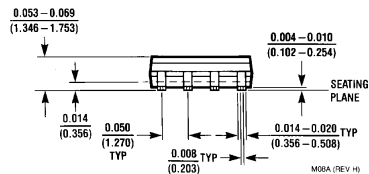
8-Pin Small Outline Package Order Number LMC7211AIM, LMC7211AIMX, LMC7211BIM or LMC7211BIMX NS Package Number M08A
