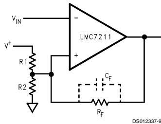
FIGURE 4. Positive Feedback for Hysteresis
