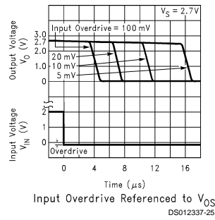
Response Time for Various Input Overdrives -t_{PHL}
