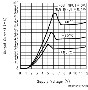
Output Sinking Current vs Supply Voltage
