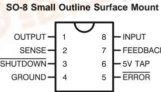
Top View Order Number LP2954AIM or LP2954IM See NS Package M08A
