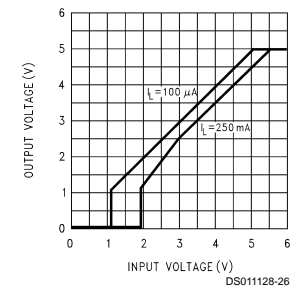
Dropout Characteristics
