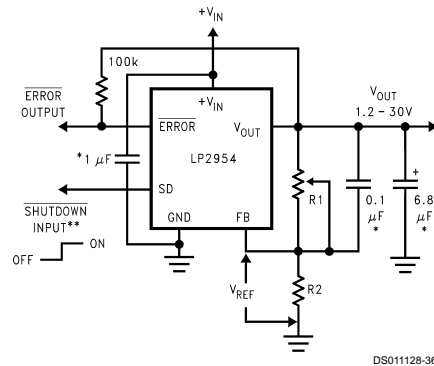
FIGURE 2. Adjustable Regulator
