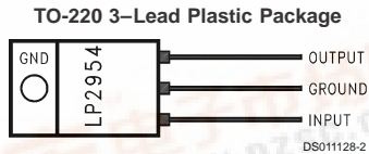
Front View Order Number LP2954AIT or LP2954IT See NS Package T03B
