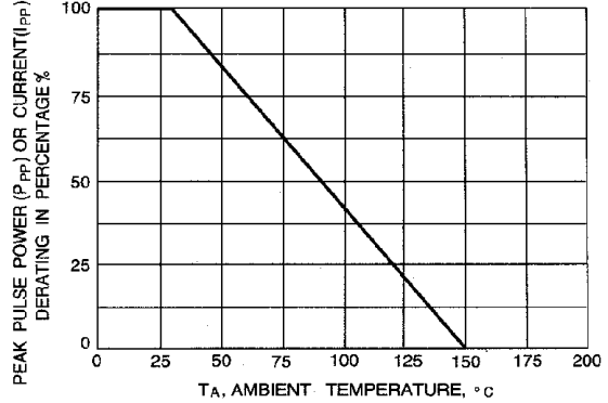
FIG.2-PULSE RATING CURVE
