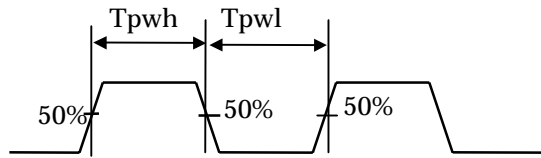
Fig.7 Clock timing
