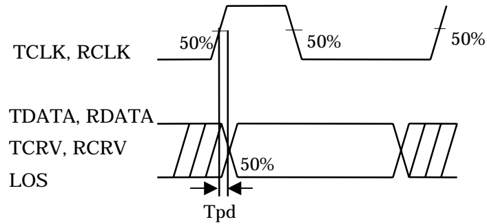
Fig.8 Transmitter Timing
