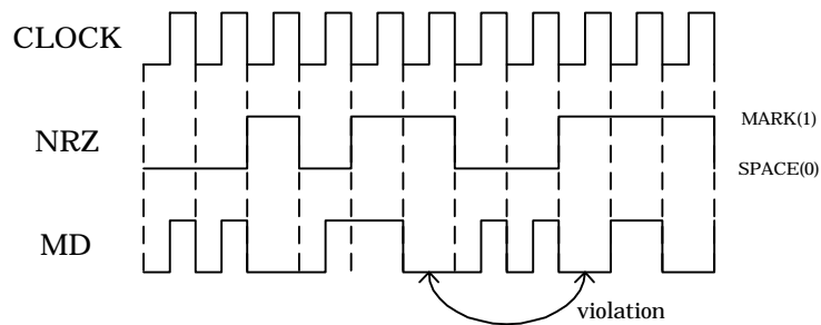
Fig.10 MD code
