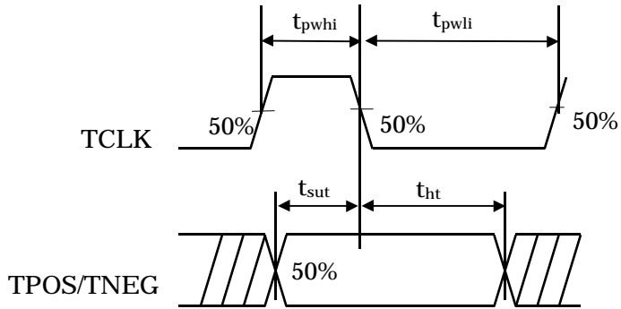
Fig. 2 Transmitter Timing
