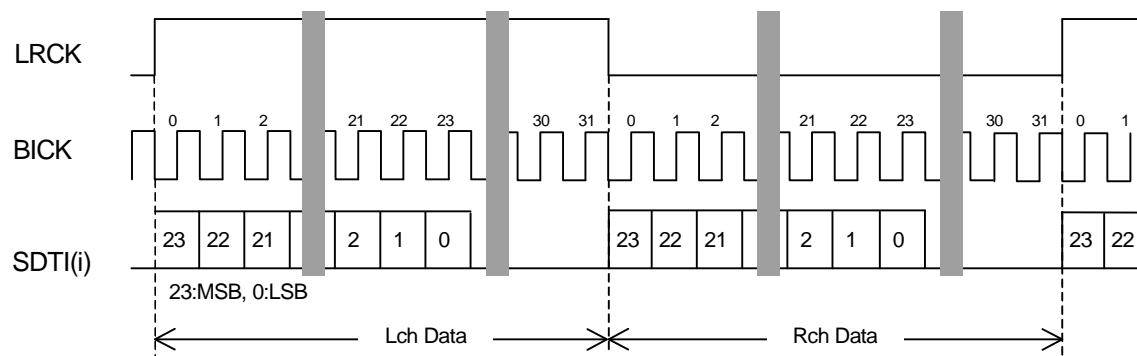
Figure 12. Mode 4, 6 Timing
