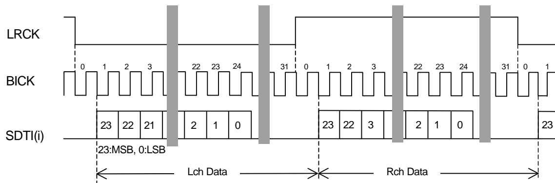
Figure 13. Mode 5, 7 Timing
