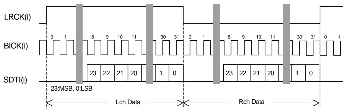
Figure 11. Mode 3 Timing
