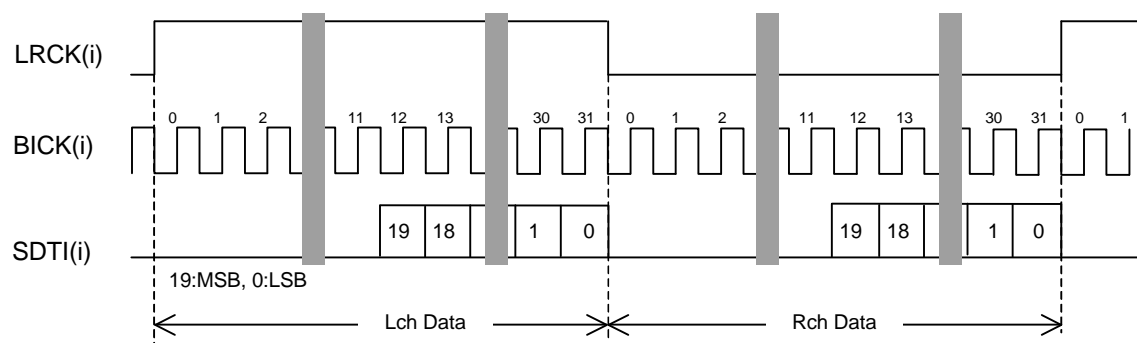
Figure 10. Mode 2 Timing
