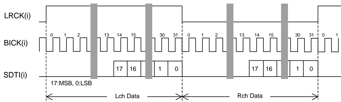
Figure 9. Mode 1 Timing
