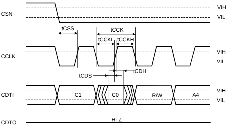
Figure 3. WRITE/READ Command Input Timing
