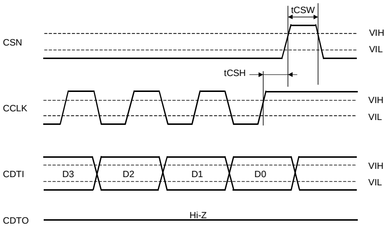
Figure 4. WRITE Data Input Timing
