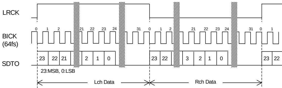
Figure 22. Mode 4 Timing
