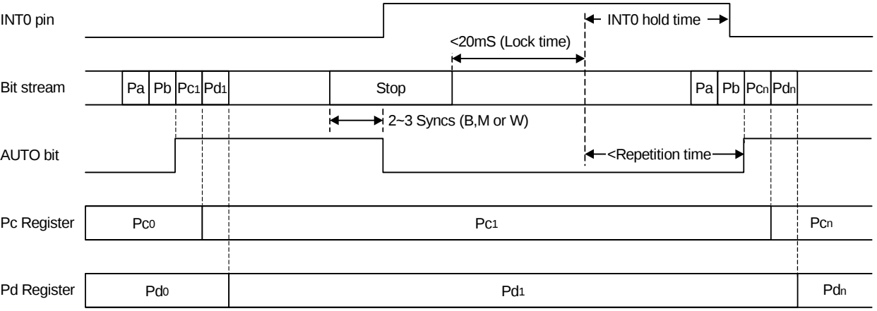
Figure 28. Timing example 2
