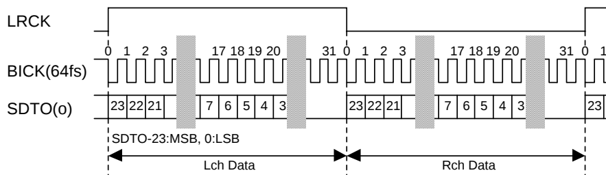
Figure 10. Mode 0 Timing
