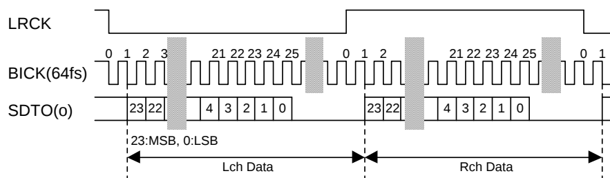
Figure 11. Mode 1 Timing
