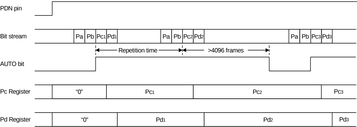
Figure 27. Timing example 1
