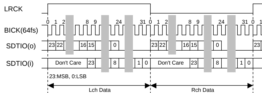
Figure 9. Mode 3 Timing
