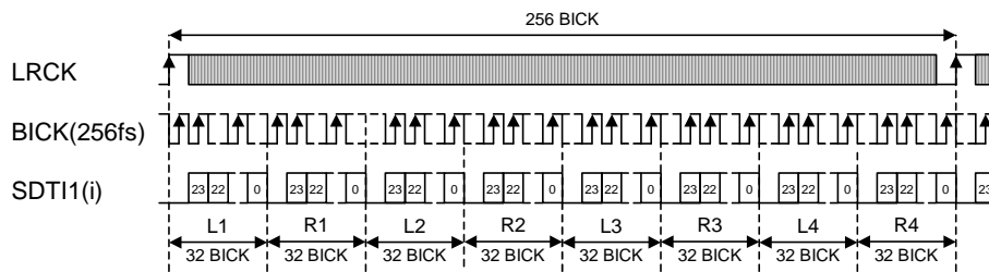
Figure 7. Mode 7 Timing
