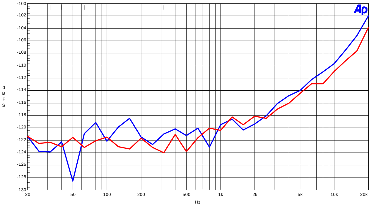
AKM (ADC fs=44.1kHz) AK4527 Crosstalk
