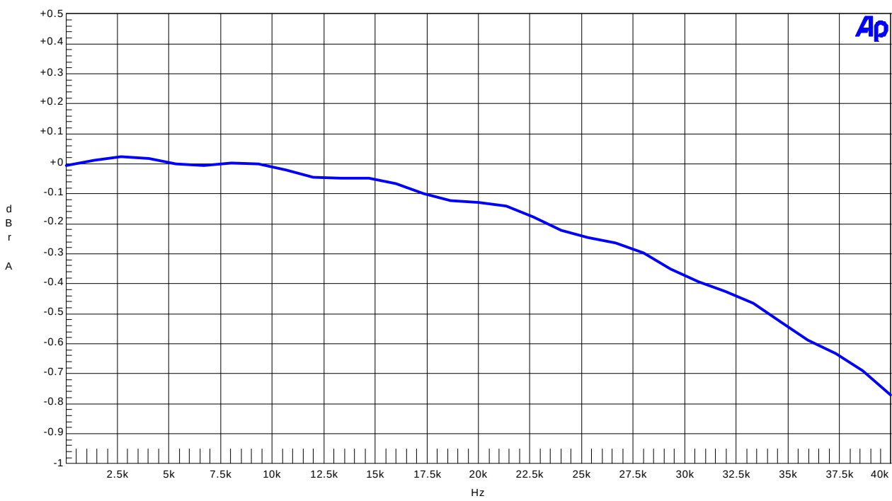
Frequency Response(Input Level=0dBFS) (including external RC filter) AK4527 Crosstalk
