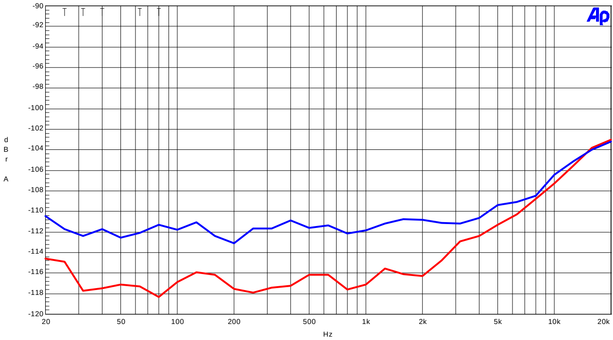
Crosstalk(Upper=Rch, Lower=Lch)
