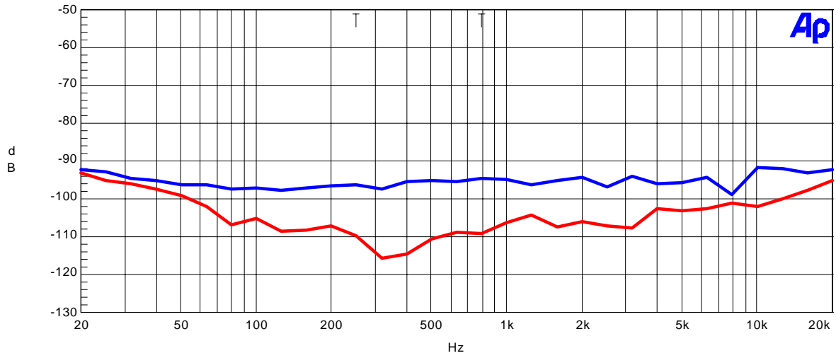
Fig5. Crosstalk
