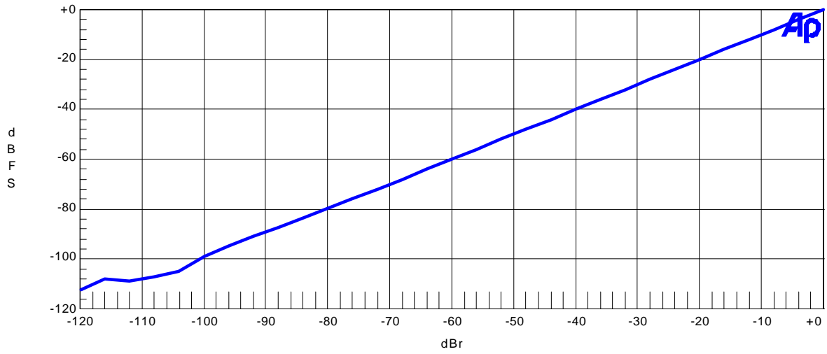
Fig3.Linearity
