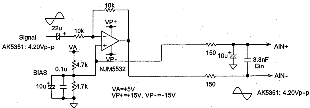
Figure 3. Single-ended Input Buffer Circuit example
