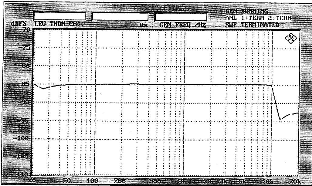
THD+N vs. Frequency
