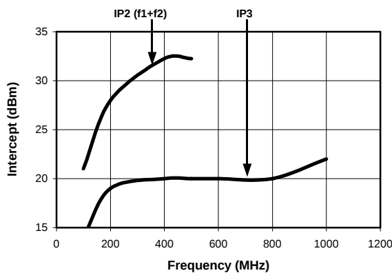
Intermodulation Intercept
