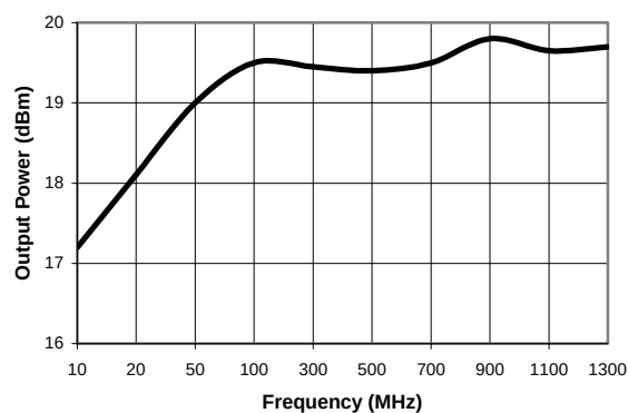
1 dB Compression
