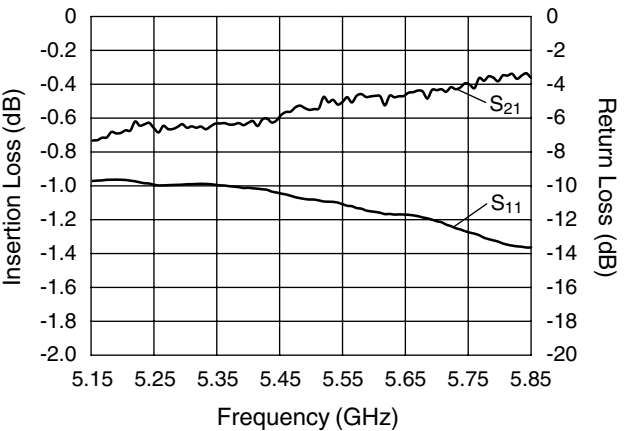
IN 1 to HP1, In Band
