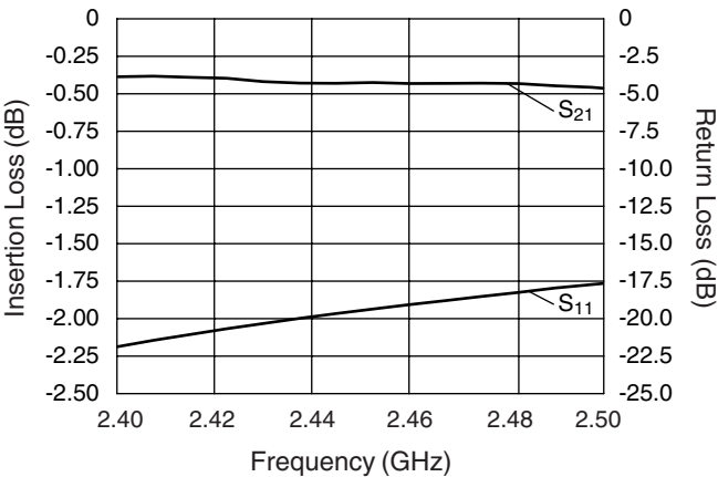
IN 1 to LP1, In Band
