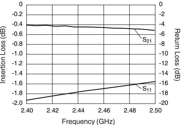
IN 2 to LP2, In Band
