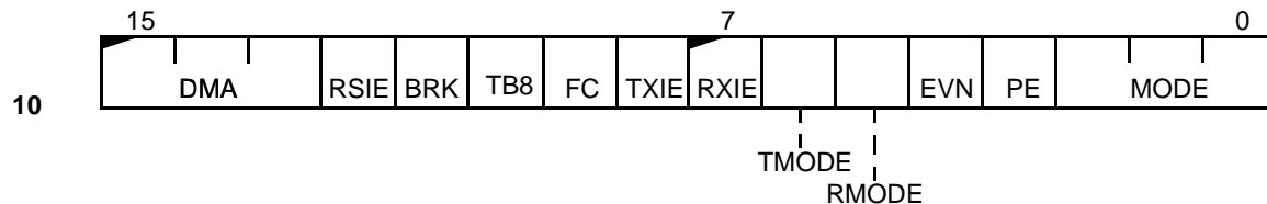
Serial Port 1 Control Register (SP1CT) Page 10-5
