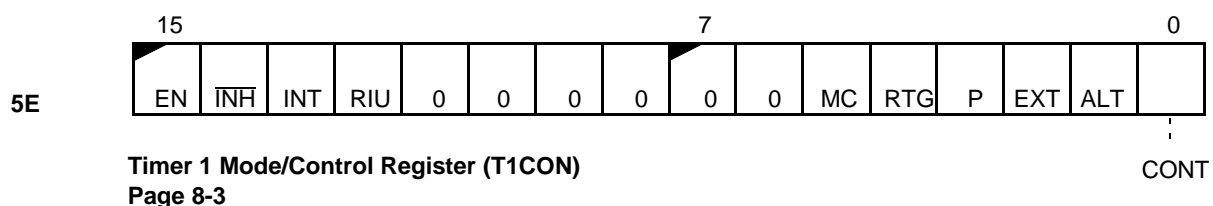
Figure A-1 Internal Register Summary (continued)
