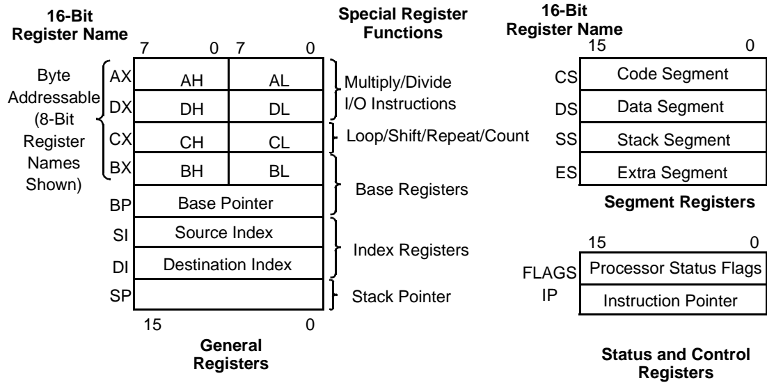
Figure 2-1 Register Set
