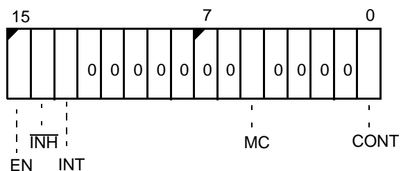
Figure 8-3 Timer 2 Mode and Control Register
