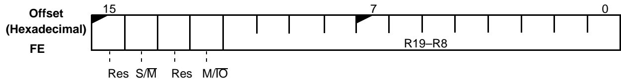
Peripheral Control Block Relocation Register (RELREG) Page 4-3
