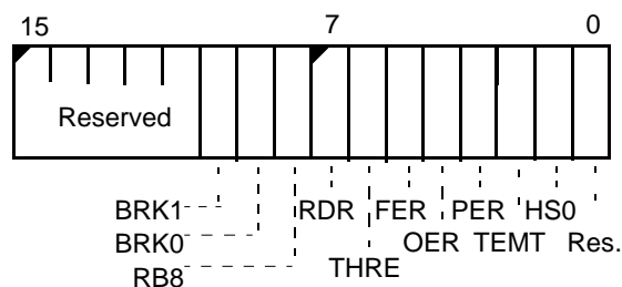
Figure 10-4 Serial Port 0/1 Status Register
