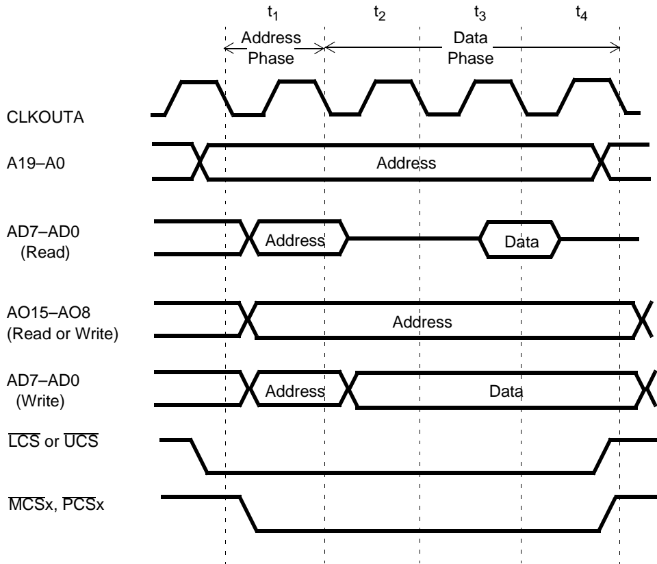
Figure 3-3 Am188ES Microcontroller Address Bus—Normal Read and Write Operation
