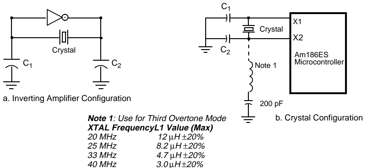
Figure 3-5 Oscillator Configurations
