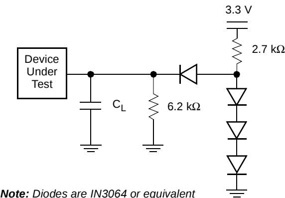
Figure 11. Test Setup
