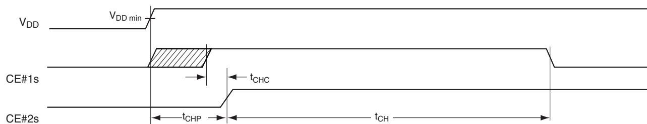
Figure 35. Power-on Timing
