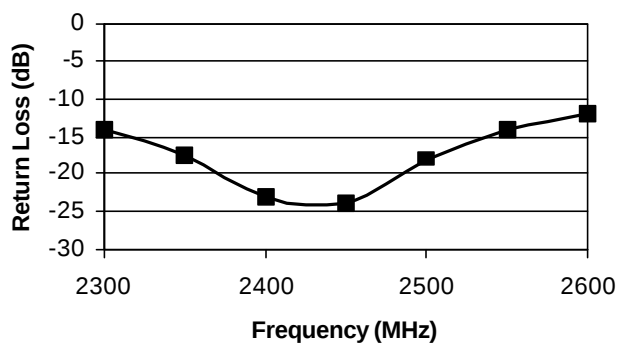
Input Return Loss, Low Power Mode
