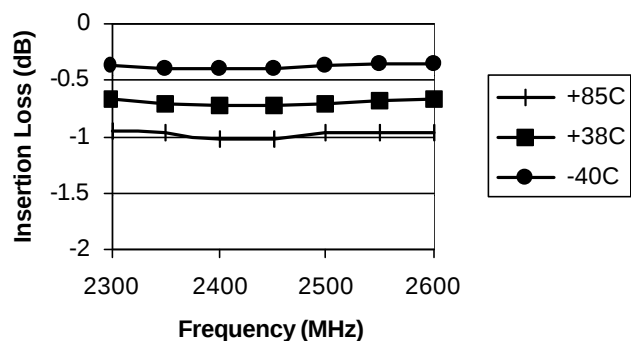
Switch Insertion Loss
