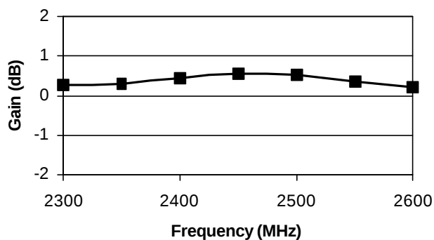
Gain, Low Power Mode
