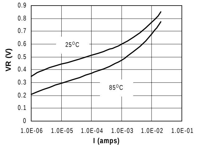
Forward Characteristic
