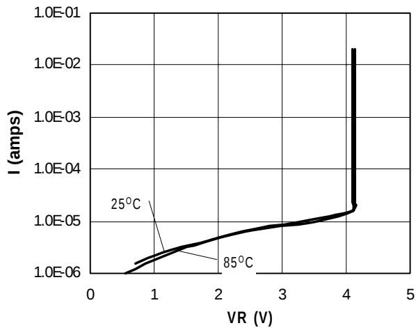
Reverse Characteristic
