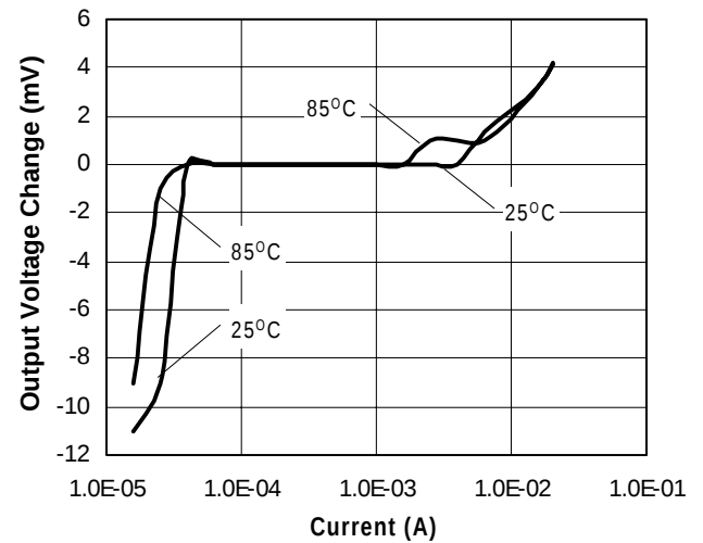
Forward Characteristic
