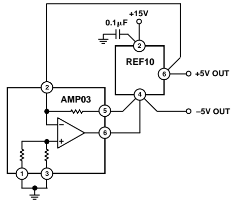
Figure 24. ±5 V Precision Voltage Reference
