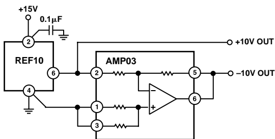
Figure 23. ±10 V Precision Voltage Reference
