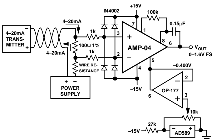
Figure 13. 4-to-20 mA Line Receiver
