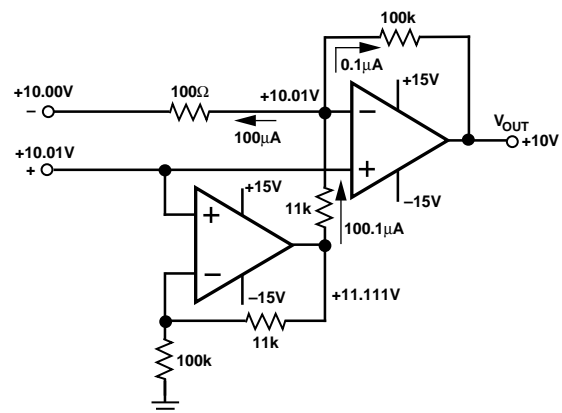
Figure 4. Gain = 1000, AMP04
