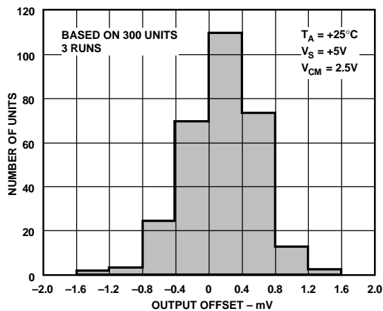
Figure 20. Output Offset ( V_{oot} ) Distribution @ +5 V
