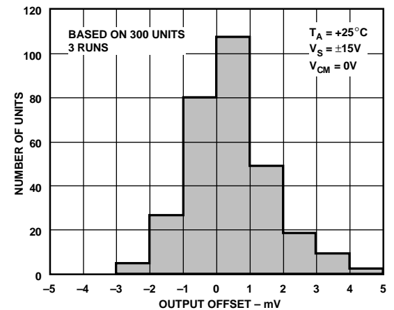
Figure 21. Output Offset ( V_{oot} ) Distribution @ \pm 15 V
