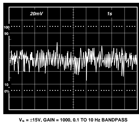
Figure 37. Input Noise Voltage
