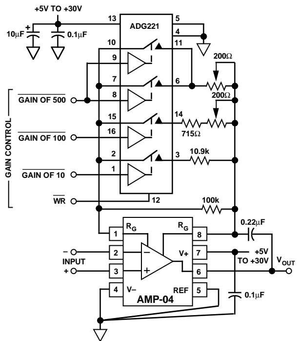
Figure 15. Single Supply Programmable Gain Instrumentation Amplifier
