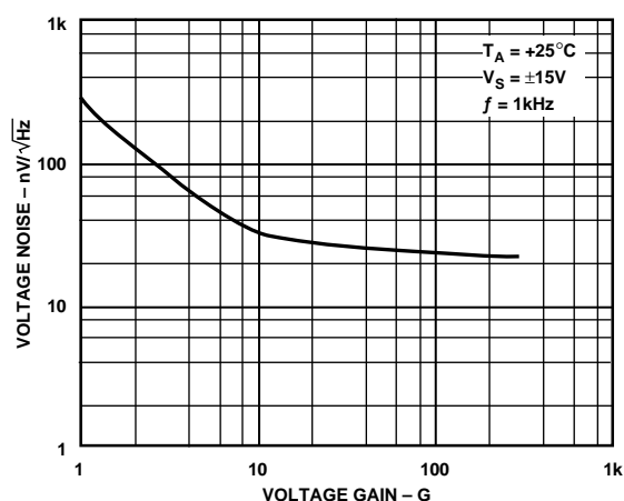
Figure 35. Voltage Noise Density vs. Gain, f = 1\text{kHz}
