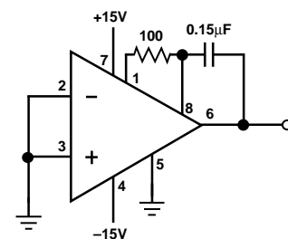
Figure 7a. 10 Hz Low-Pass Filter
