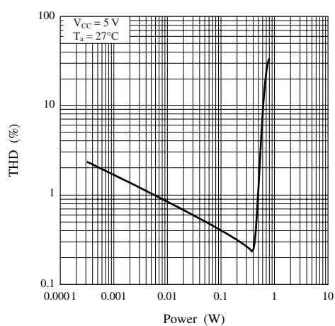
THD — Power
