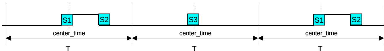
Figure 8. svmStdDtXor_sync timing
