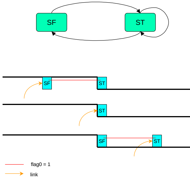
Figure 5. svmStdDtXor_T state diagram and 3 cases of timing
