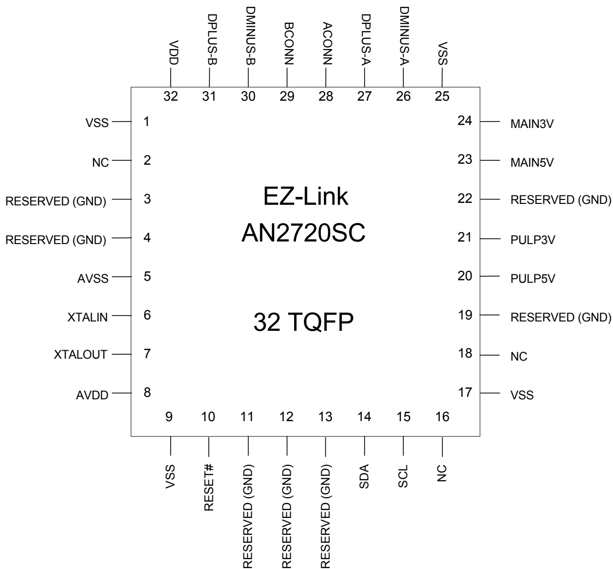
Figure 1. AN2720SC pinout
