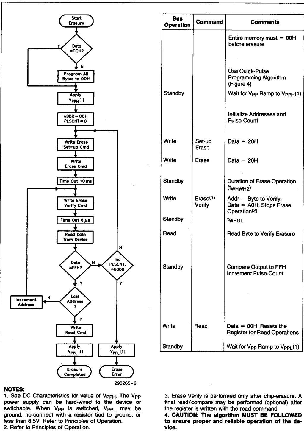
Figure 5 28F512 Quick-Erase Algorithm
