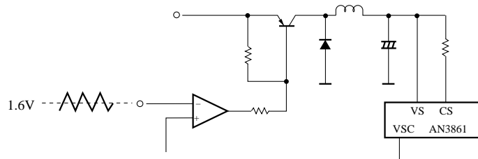
Fig.3 Switching Regulator System with VSC Terminal
