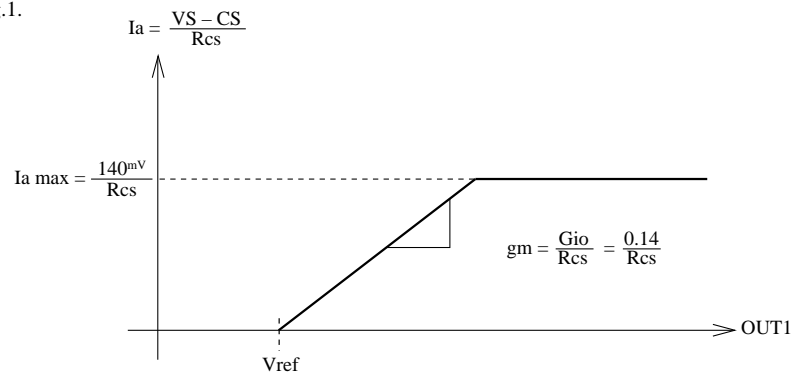
Fig.1 Drive Characteristics
