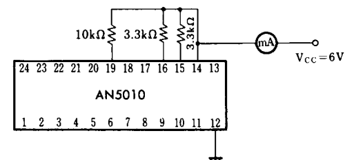
Test Circuit 16 ( I_{Lo} )
