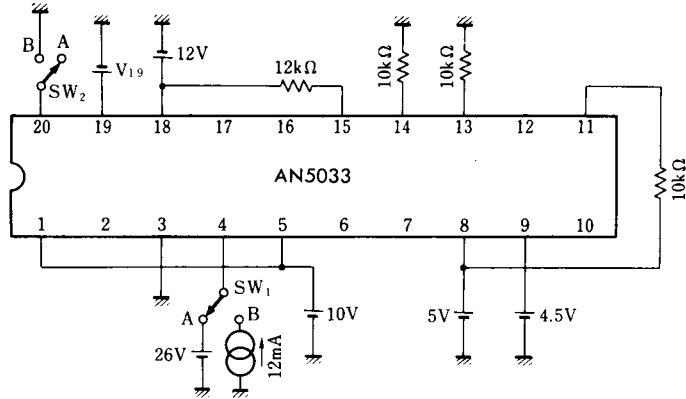
Test Circuit 2 ( I_{15} , V_{12-3(2)} , V_{12-3(3)} , V_{12-8} , V_{13,14,15,16,17-3} )
