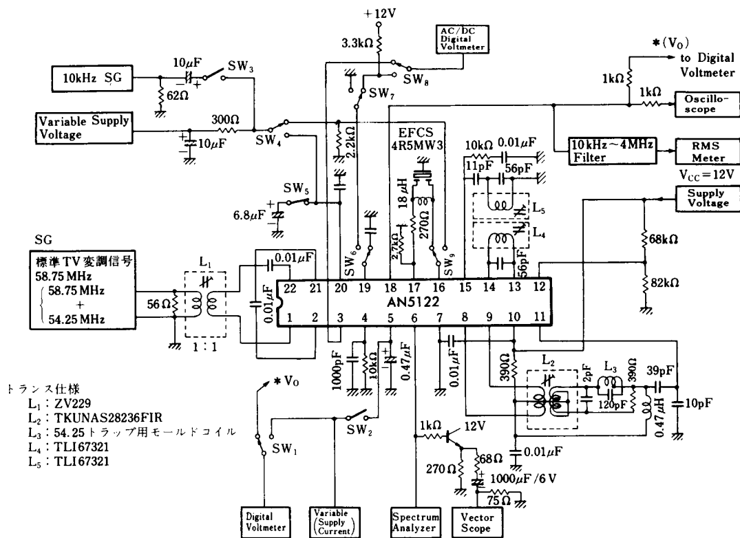
Test Circuit 5 ( G_{V(2)} , V_{O(1)} , S_{(IN)} , R_{AGC} , V_{O(2)} )
