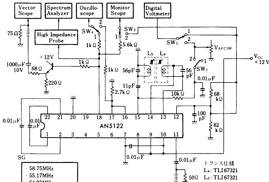
Test Circuit 3 ( V_i, DG, DP, f_c, \mu )
