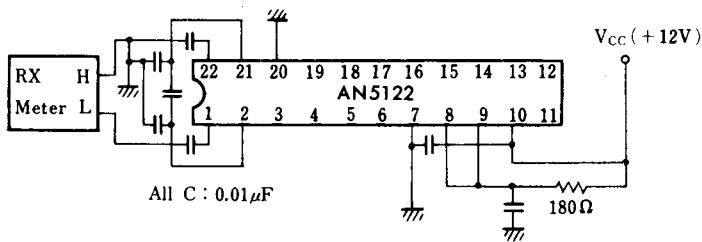
Test Circuit 3 ( V_i, DG, DP, f_c, \mu )
