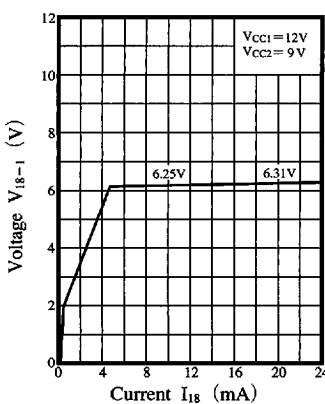
Zener Characteristics (1)
