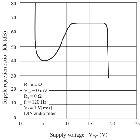
RR — V_{CC}
