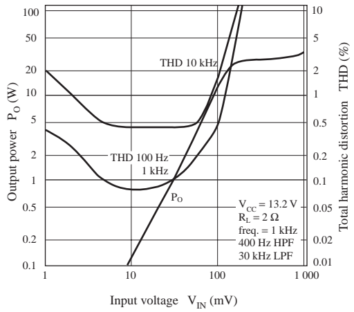
P_O, THD - V_{IN} (R_L = 2 \Omega)
