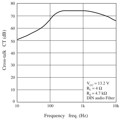
CT — freq.
