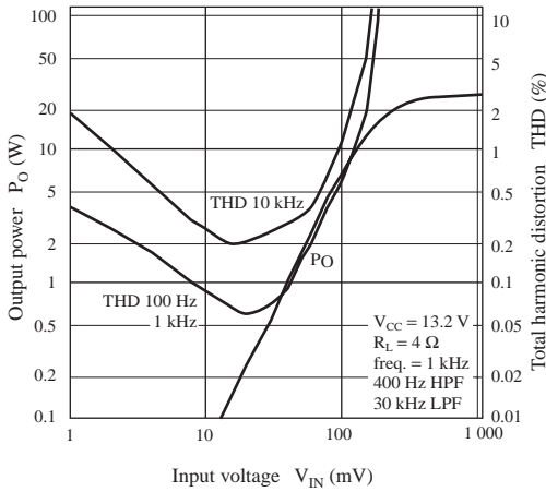
P_O, THD - V_{IN} (R_L = 4 \Omega)
