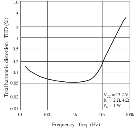
THD — freq.
