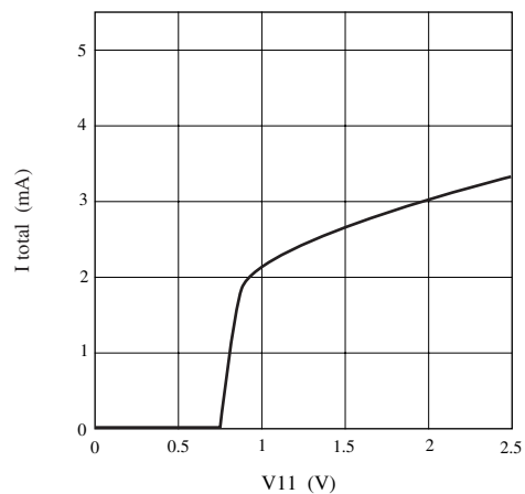
12. V_{CC} - I_{total}
