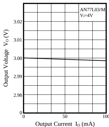
Load Stability V_O - I_O
