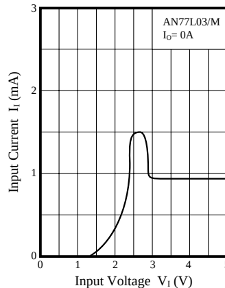
Rush Current (Under No Load) I_I - V_I
