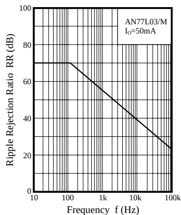
Ripple Rejection Ratio \text{RR} - f
