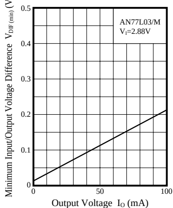
Minimum Input/Output Voltage Difference V_{\text{DIF (min)}} - I_{\text{OUT}}
