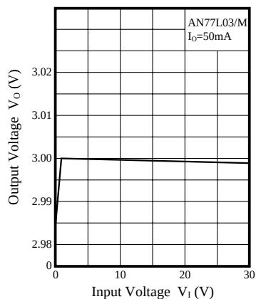
Input Stability V_O - V_I
