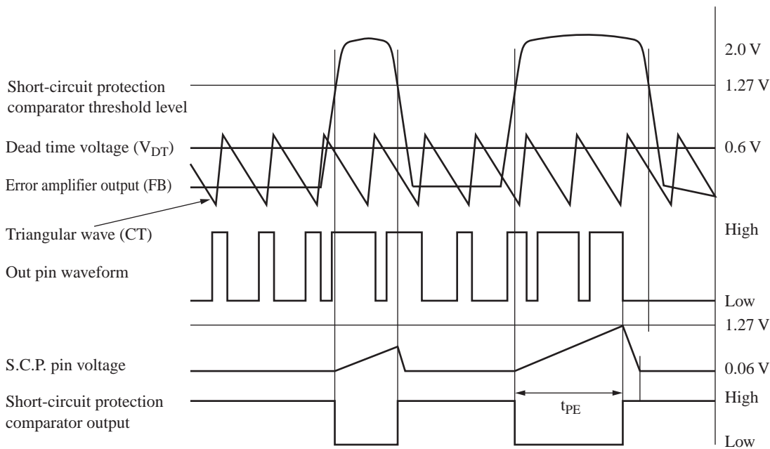
Figure 2. Short-circuit protection operating waveforms
