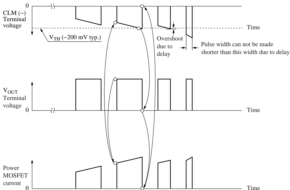
Figure 6. Pulse-by-pulse overcurrent detector operation waveform
