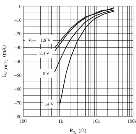
R_B — I_{SO(OUT)}
