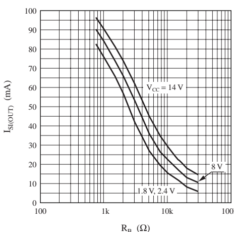
R_B — I_{SI(OUT)}
