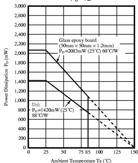
P_D – T_a
