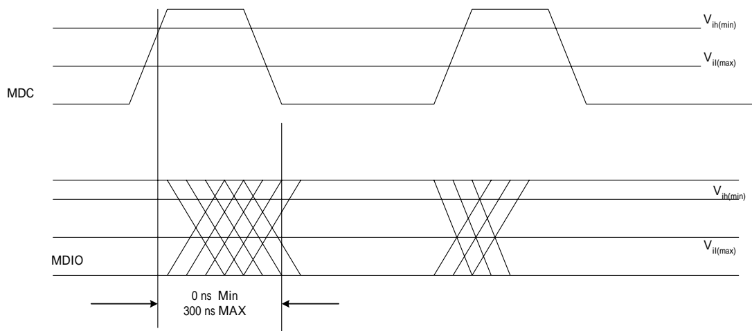
FIG- 24 MDIO SOURCED BY PHY
