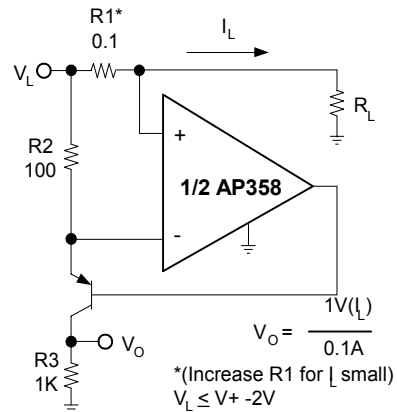
Current Monitor
