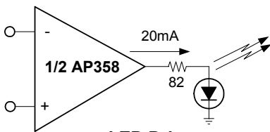
LED Driver
