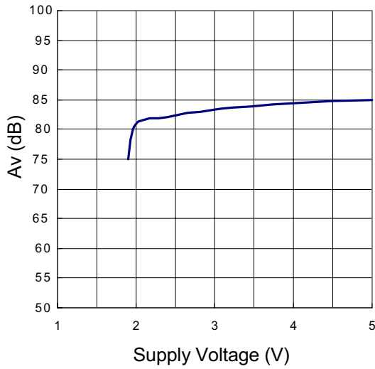
Large Signal Voltage Gain vs Supply Voltage
