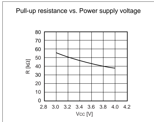
(4) Pull-up resistance
