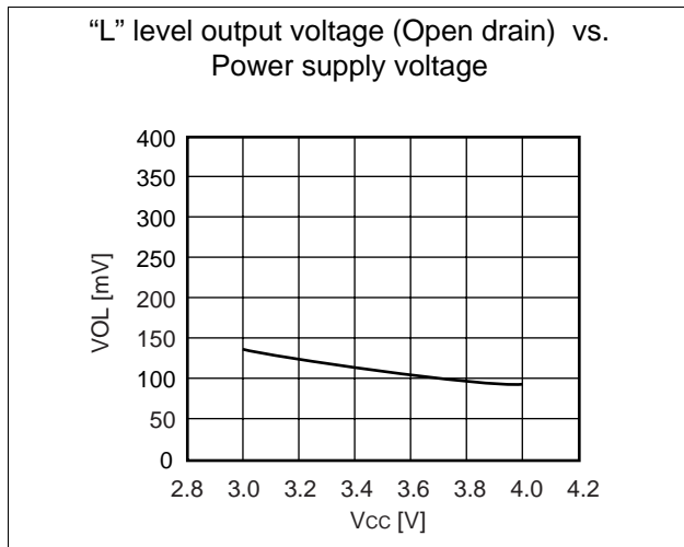
(3) "L" level output voltage (Open drain)
