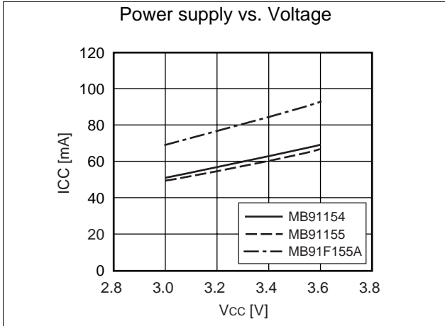
(5) Power supply
