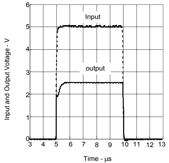
Pulse Response
