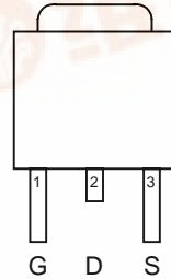
Top View of TO-252
