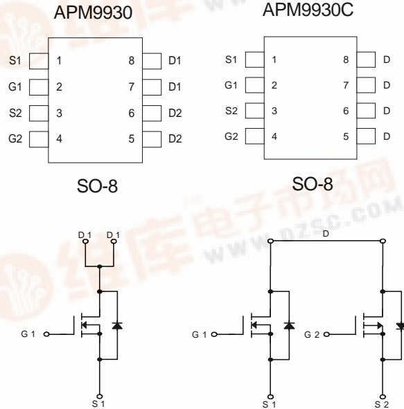
N-Channel MOSFET
